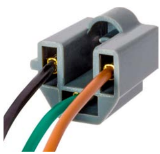
23035 (88860446, 12117333) Sealed Beam Headlights Socket Assembly With Fiber Optics Gauge: 16 Three GPT 8" Leads GM
