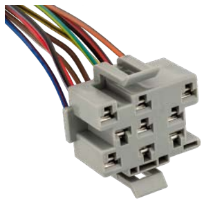
17624 (Not Supplied by O.E.M.) Headlight Switch Assembly Harness Connector Fits Instrument Panel Headlight Switch E7TZ-11654-C Ford Trucks: F150, F250, F350 & Bronco 1991-87
