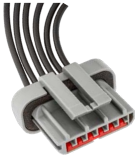
18217 (E5ZZ-12A209A) Ignition Module & Neutral Safety Switch Harness Connector For E.E.C. IV Ignition 1995-83 Ford Neutral Safety Switch E80Z-7A247-A 1988-On
