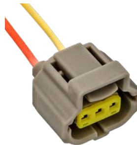
23098 (Not Available from OEM) Alternator Repair Harness Connector Gauge: 16 Two TXL 8" Leads Ford F250/350 7.3 Diesel Eng. & Cr. Vic, Gr. Marquis, Town Car, Contour & Mystique 1996 - On
